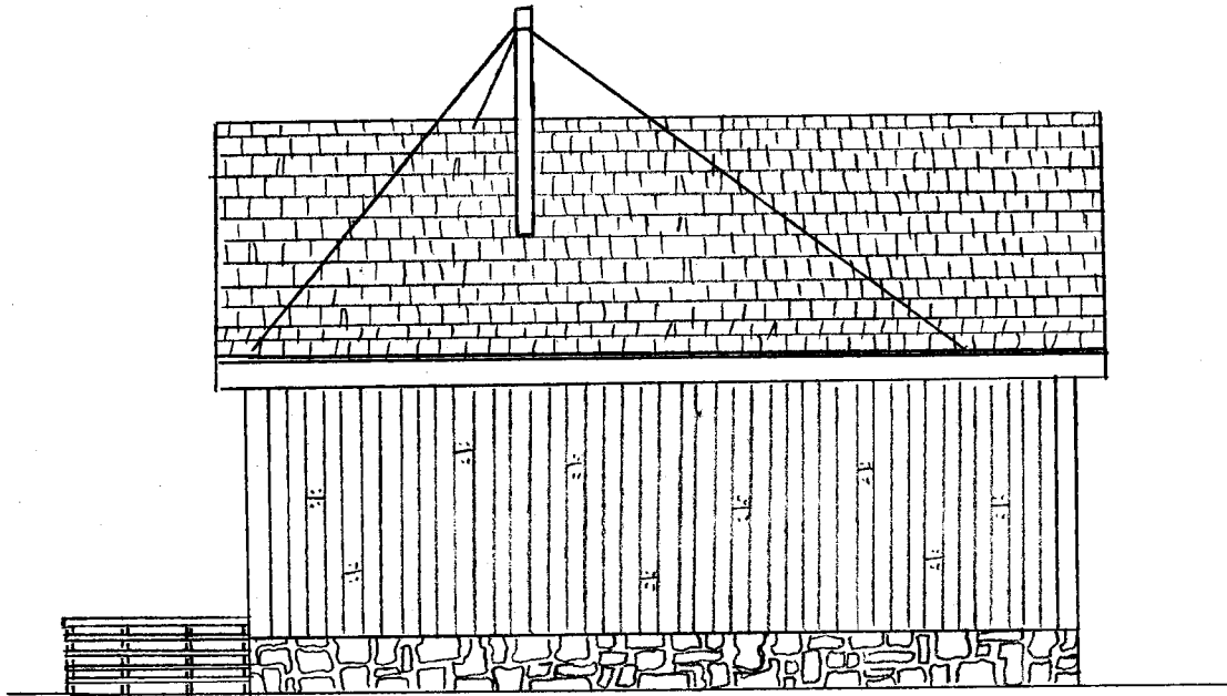
LEFT ELEVATION HD SCALE
